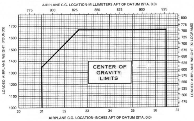
Figure 6-9. Center of Gravity Limits
